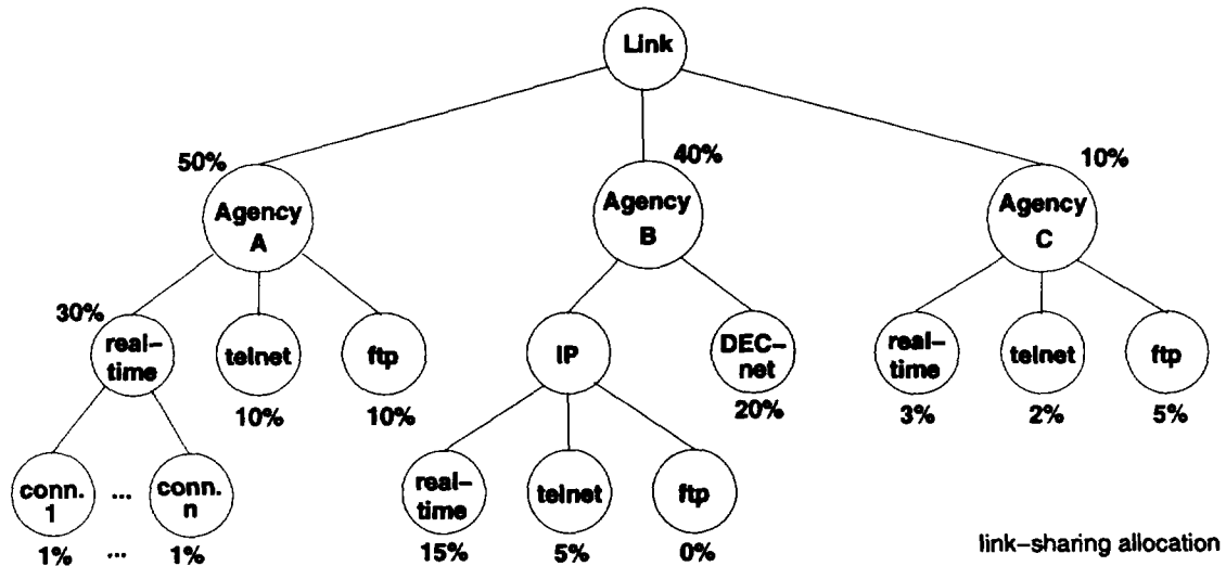
Fig. 3. A hierarchical link-sharing structure.
