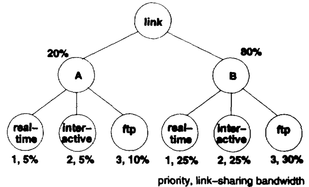
Fig. 16. Link-sharing structure for the congested gateway.
