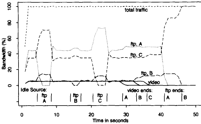
Fig. 14. Three-agency link-sharing with Top-Level link-sharing guidelines.
