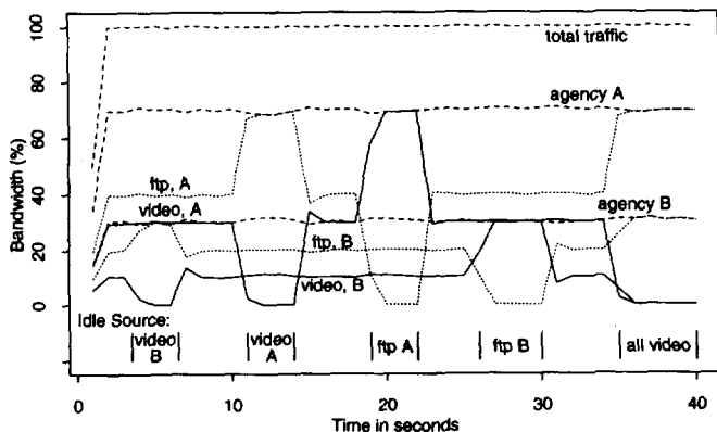
Fig. 11. Two-agency link-sharing with formal link-sharing guidelines.
