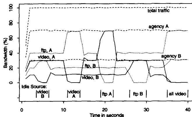
Fig. 13. Two-agency link-sharing with Top-Level link-sharing guidelines.
