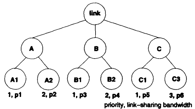
Fig. 22. Example link-sharing structure.
