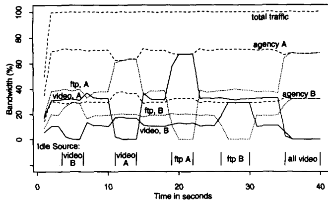
Fig. 12. Two-agency link-sharing with Ancestor-Only link-sharing guidelines.
