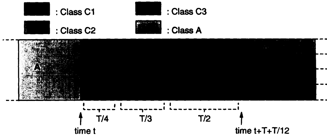
Fig. 21. Class A denied bandwidth for T + T/12 seconds.
