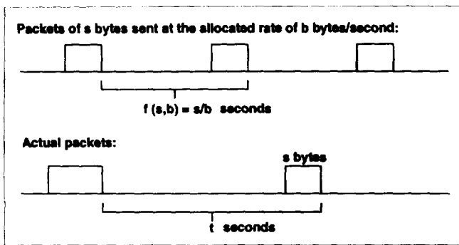
Fig. 20. Variables for the computation of the limit status of a class.
