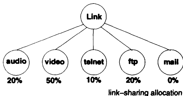
Fig. 1. Link-sharing between service classes.
