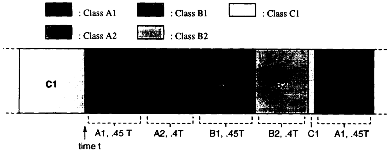
Fig. 23. Class C2 denied bandwidth indefinitely, with Ancestor-Only link-sharing.
