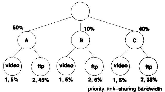
Fig. 9. Link-sharing structure for the simulation of three-agency link-sharing.
