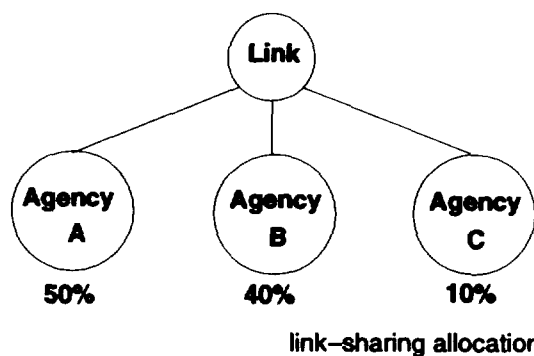
Fig. 2. Link-sharing between multiple agencies or protocol families.
