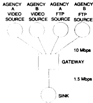
Fig. 6. Simulation scenario for two-agency link-sharing.
