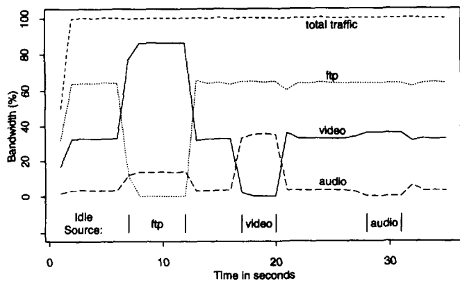
Fig. 10. Flat link-sharing with Top-Level link-sharing guidelines.
