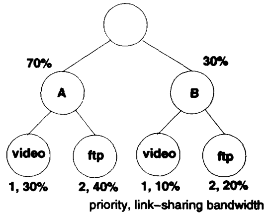
Fig. 8. Link-sharing structure for the simulation of two-agency link-sharing.
