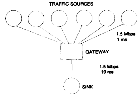
Fig. 15. General simulation scenario for the investigation of delay.
