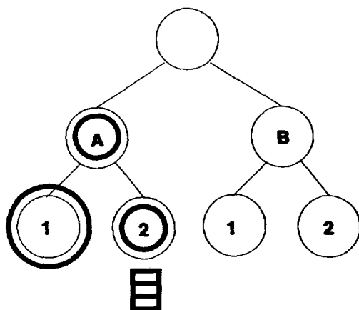
Fig. 5. Sensitivity of Ancestors-Only link-sharing.
