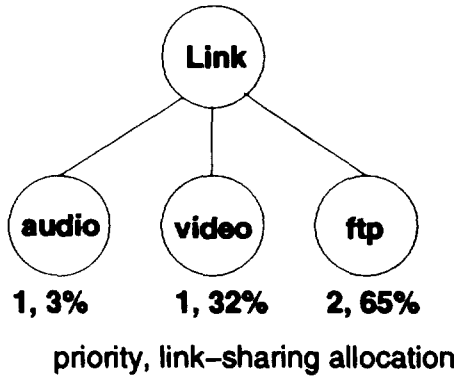
Fig. 7. Link-sharing structure for the simulation of flat link-sharing.
